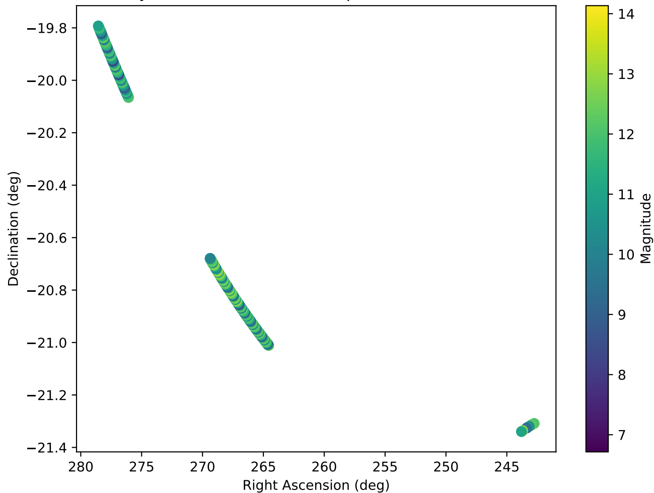
Sky Positions of PAN Telescope Detections (ICRF)
