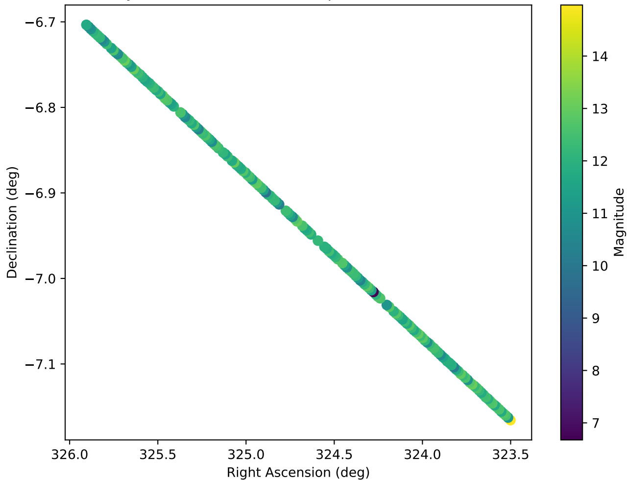
Sky Positions of PAN Telescope Detections (ICRF)
