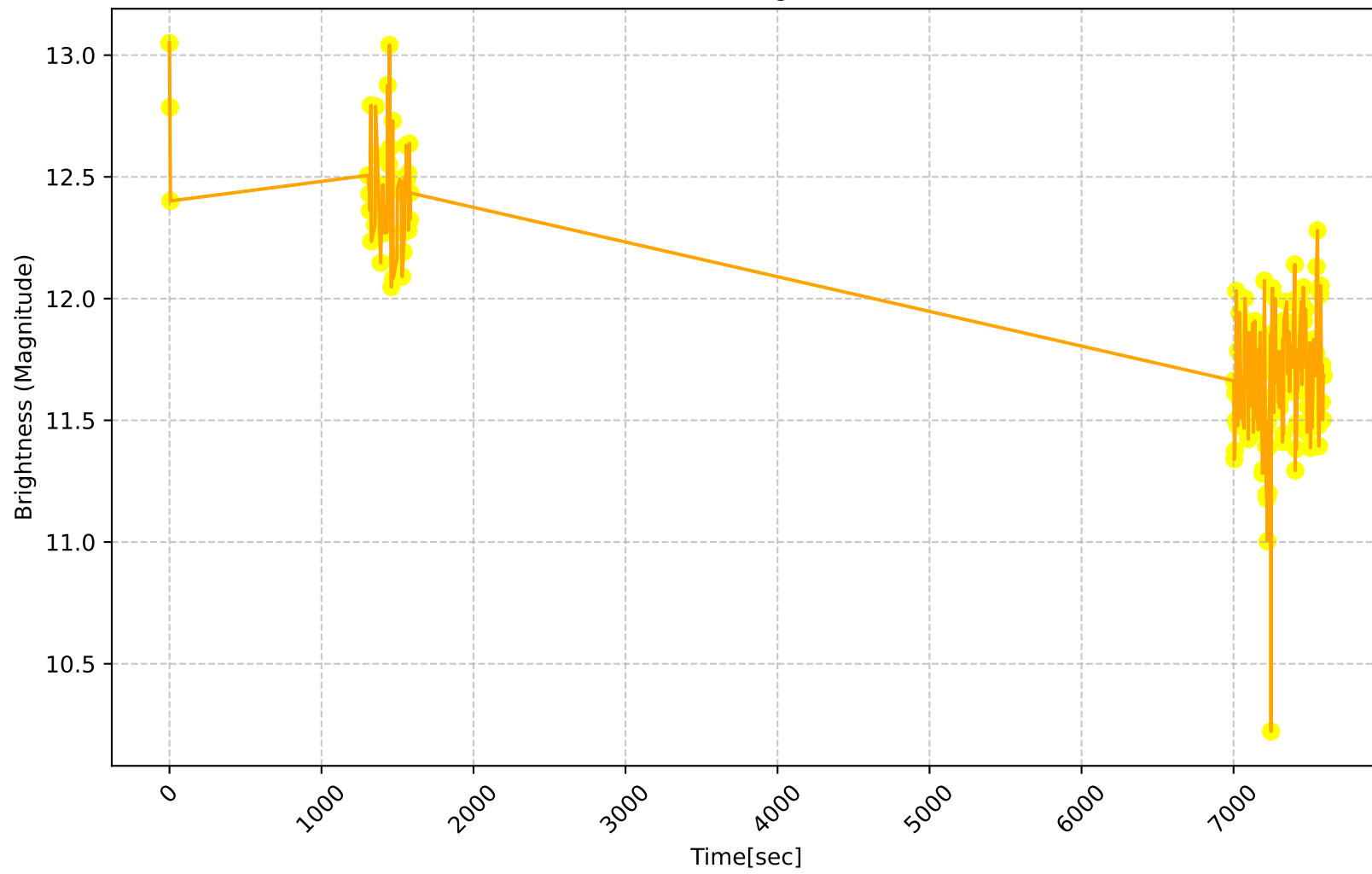
Time vs. Brightness
